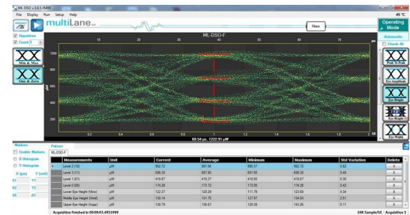
Figure 6: PAM4
