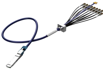
Figure 1 QSFP-DD to SMPM Cable Assembly
