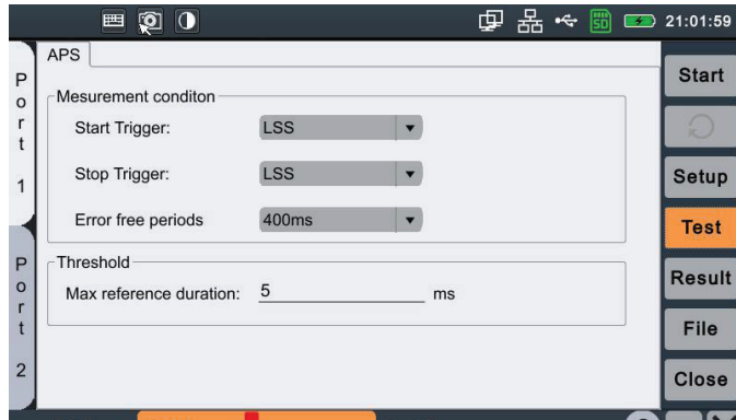
OTN APS measurement screen
