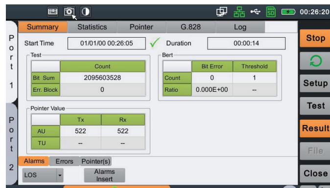
SDH Bert measurement screen
