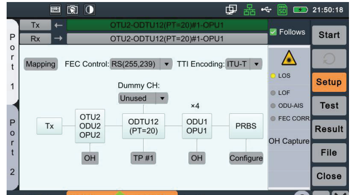
OTN BERT measurement screen.
