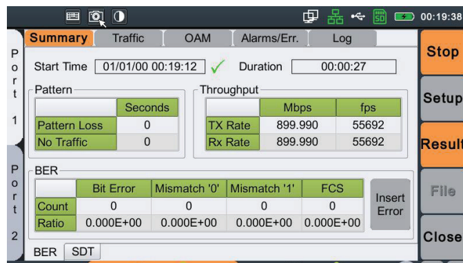
Ethernet BERT results. Click "Insert" to insert a specified number of bit/FCS errors.
