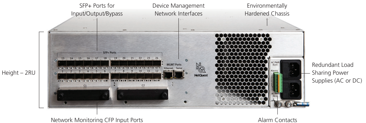
FIGURE 1 – NetQuest I-9100 100/40/10G Interceptor standard rear panel view showing key network interfaces. Interceptors are purpose-built network monitoring access solutions built on an environmentally hardened hardware platform.
