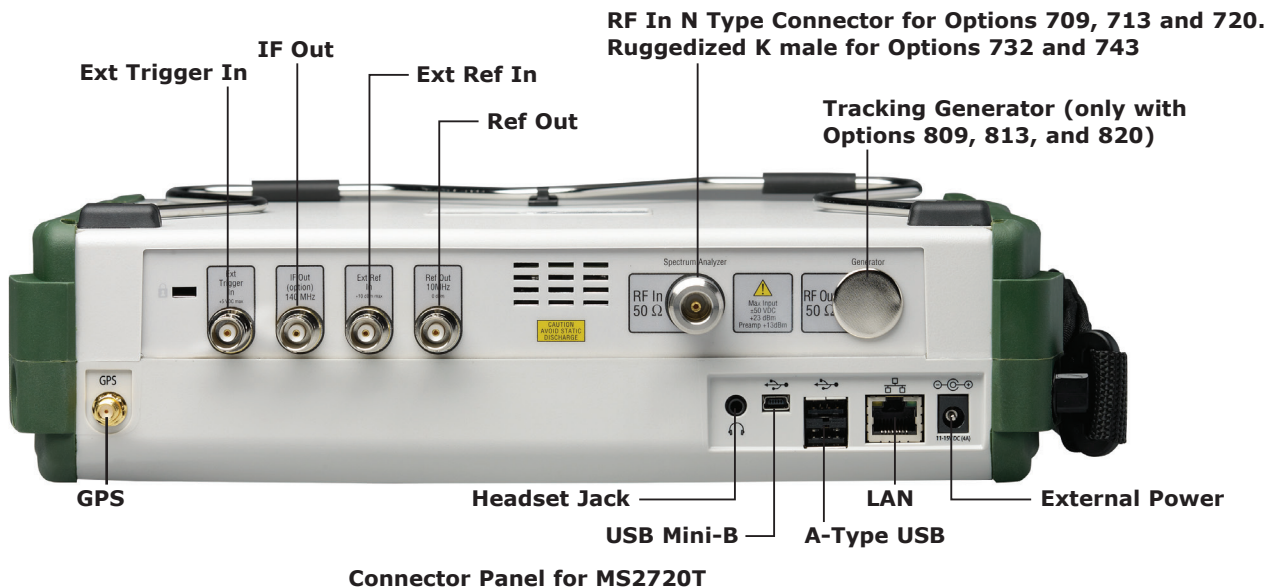
Connector Panel for MS2720T
