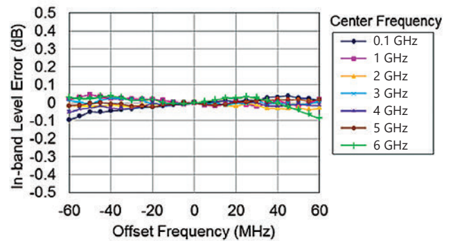
Example of frequency characteristics in analysis bandwidth after Extra Band Cal (With MS269xA-078, Reference Level: -10 dBm, Input attenuator: 10 dB, Preamp: Off, Span: 125 MHz)
